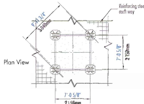
FOUNDATION DETAILS with S35 Tower Sections (Concrete Slab)
